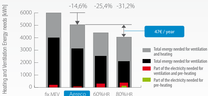
graph n.1 – Total energy consumption of various ventilation systems Assumption: 1 kWh electricity = 0.19 € ; 1 kWh Fuel or Gas = 0,07 €
