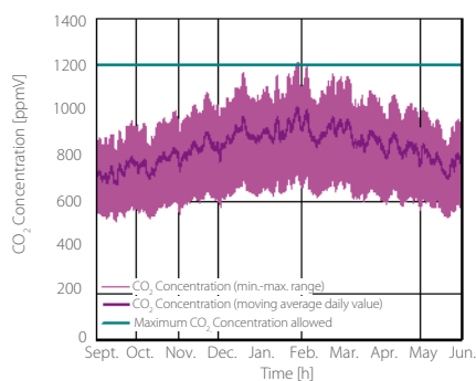
graph n.3 – Daily variation of CO 2 inside the dwelling.
