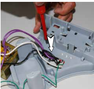
9. Remove the connectors (x 2).
